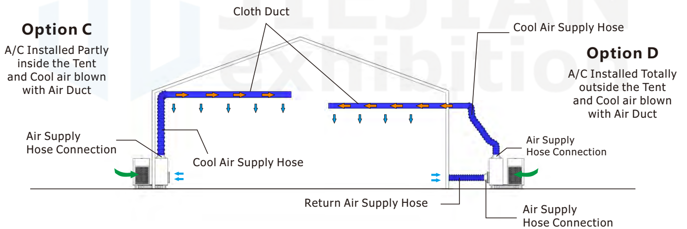
Demonstration of A/C Installed with Air Duct
